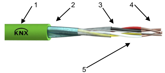
Figure 1. Câble KNX 2 x 2 x 0.8mm
